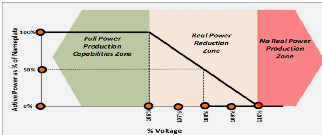
Figure Hh-3: Volt-Watt Requirements
