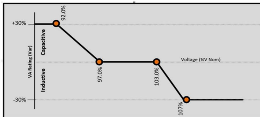
Figure Hh-1: Voltage and Reactive Default Settings
